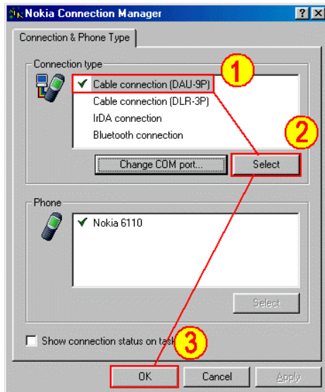
Figure 3. By clicking the Connection button the Nokia Content Copier will launch the Nokia Connection Manager. Select the connection type and phone model if several are listed.
