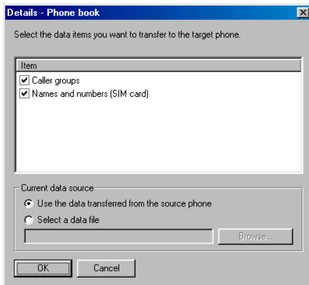
Figure 5. In the Details screen you can select the data items to be transferred to your phone, and if you wish, you can use some old data on your hard disk (must be in .CVS format) you can do so.
