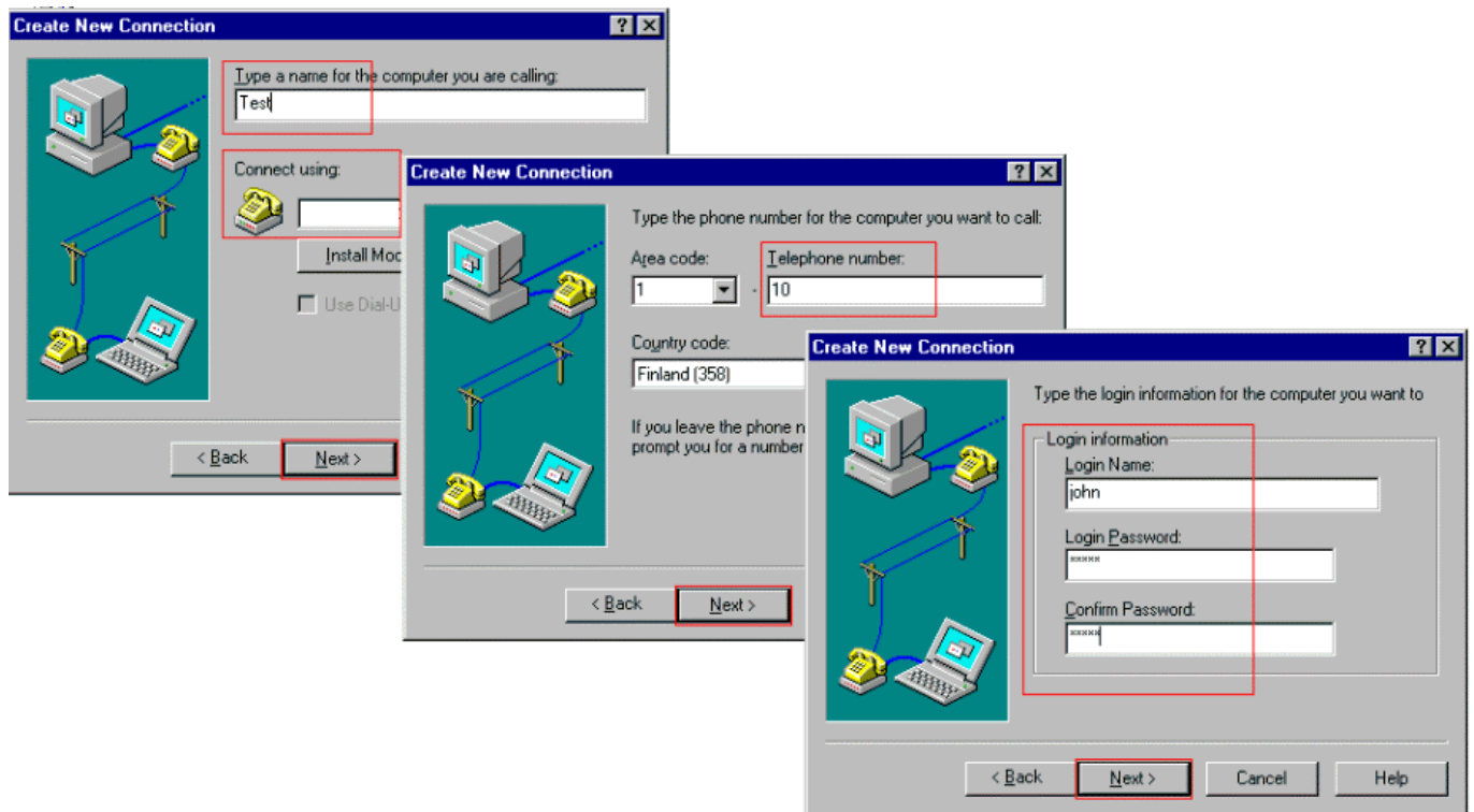
Figure 3. The first three steps towards creating a new connection.
