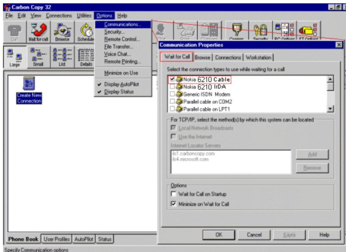
Figure 1. Accessing the program's setup and selecting the appropriate modem.
