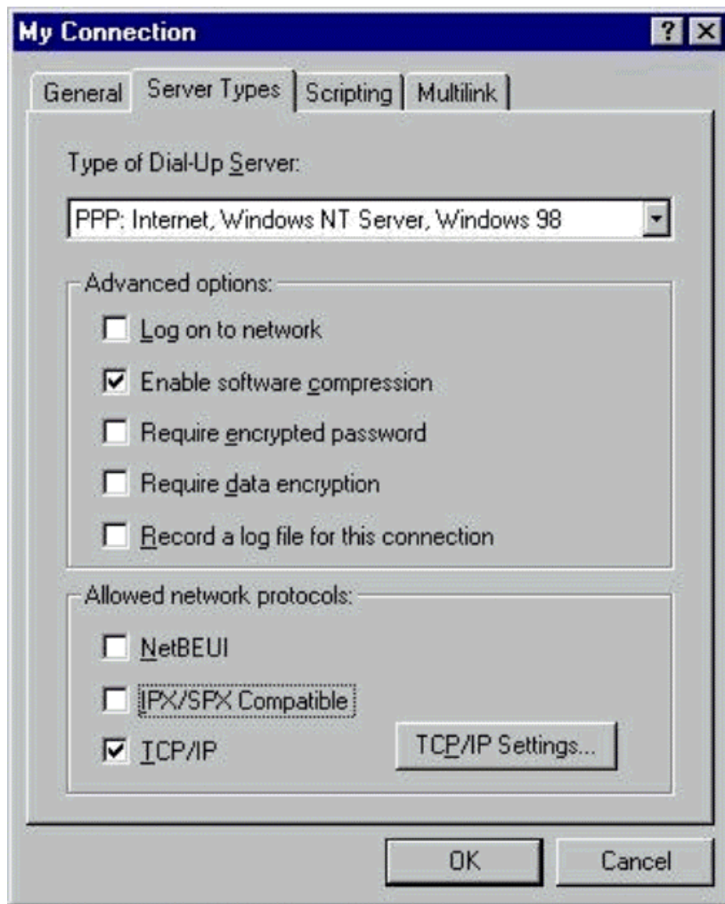
Figure 5. Server types.
