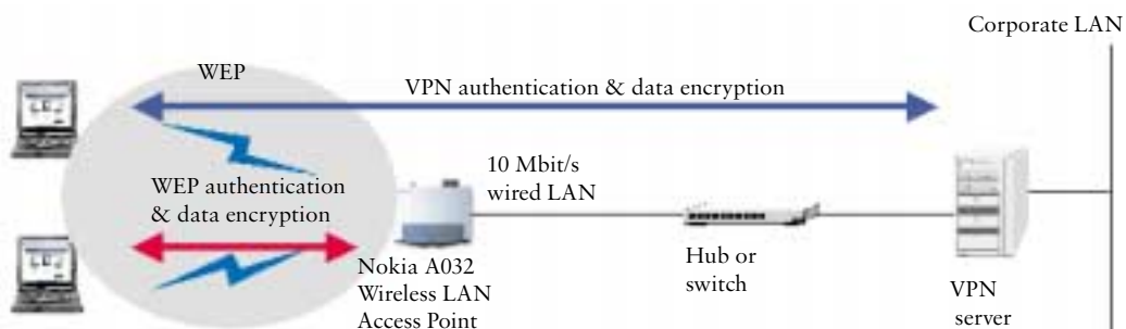
Figure 3. Example of VPN & WEP in a wireless LAN
