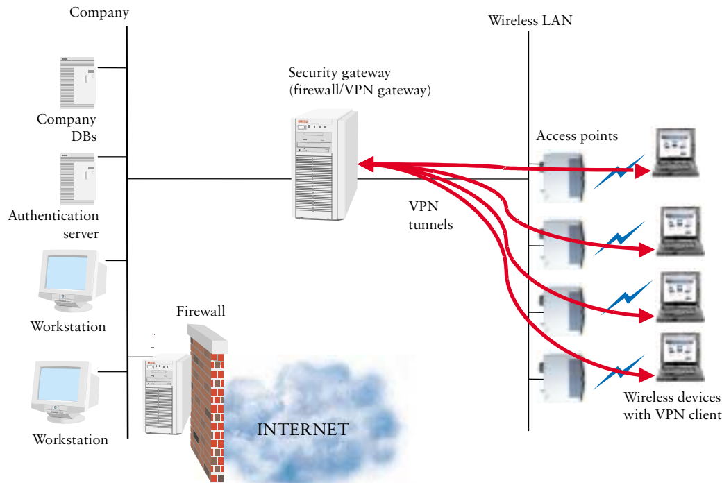
Figure 1. A wireless LAN segment in a corporation
