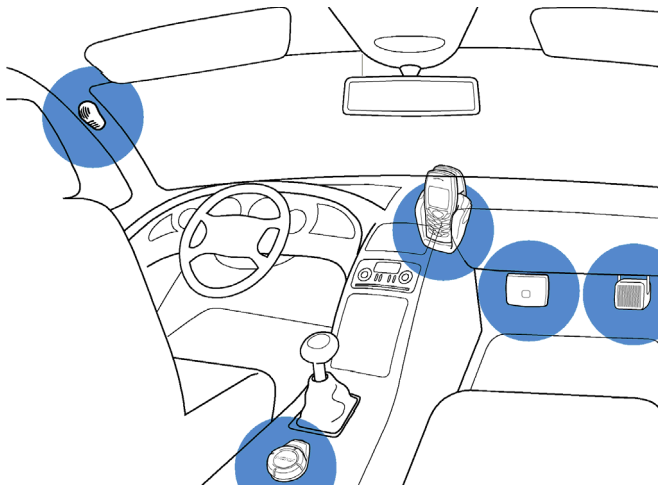
Advanced Car Kit equipment installation in the cockpit
