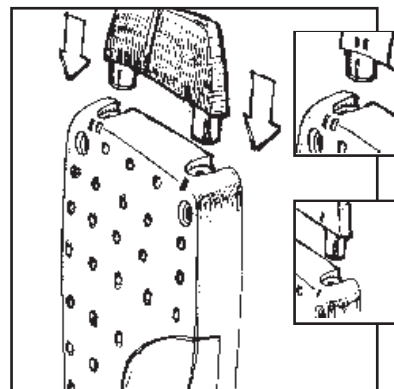
3. Connect the antenna to the terminal. Please ensure that marks I and II on both the terminal and antenna face in the right direction.
