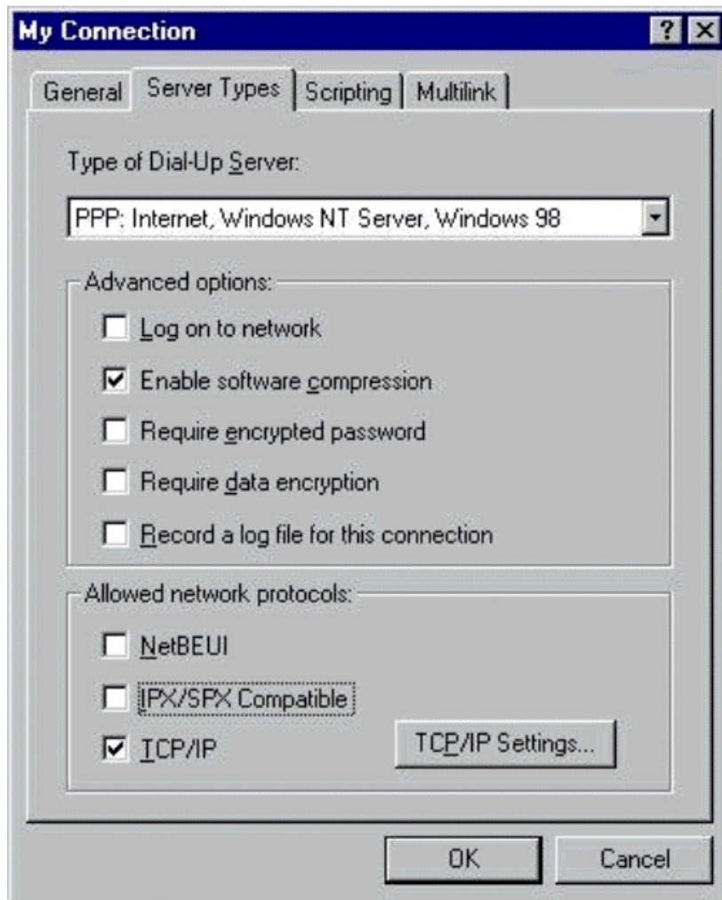
Figure 5. Server types.
